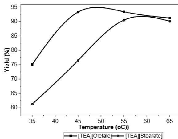
Figure 2. Influence of reaction temperature on the synthesis efficiency of [TEA][oleate] and [TEA][Stearate] (molar ratio [\text{RCOOH}]/[\text{TEA}] = 1.3 ; 6 h for [TEA][oleate] and 7 h for [TEA][Stearate]).
