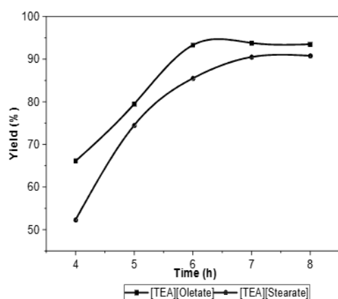
Figure 3. Influence of reaction time on the synthesis yield of [TEA][Oleate] and [TEA][Stearate] (with molar ratio [RCOOH]/[TEA] = 1.3; temperature 45 °C with [TEA][Oleate] and 55°C with [TEA][Stearate])
