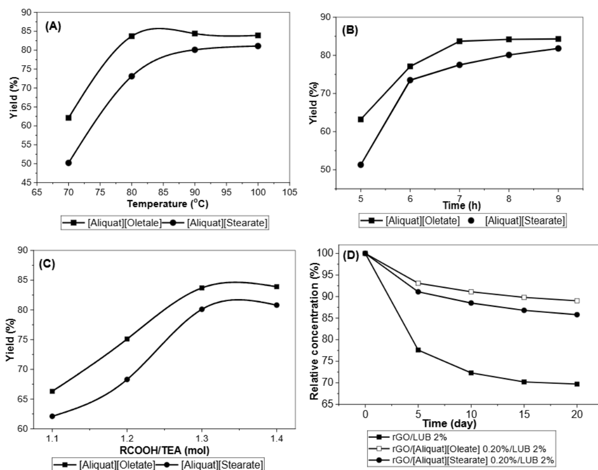
Fig. 2: Influence of (A) reaction temperature on the synthesis efficiency of [Aliquat][oleate] and [Aliquat][Stearate] (molar ratio [RCOOH]/[Aliquat]= 1.3; 7 h for [Aliquat][ oleate] and 8 h for [Aliquat][Stearate]); (B) reaction time on the synthesis yield of [Aliquat][Oleate] and [Aliquat][Stearate] (molar ratio [RCOOH]/[Aliquat]= 1.3; temperature 80 °C with [Aliquat][Oleate] and 90°C with [Aliquat][Stearate]); (C) [RCOOH]/[Aliquat] molar ratio on IL synthesis performance (7 h for [Aliquat][ oleate] and 8 h for [Aliquat][Stearate], temperature 80 °C with [Aliquat][Oleate] and 90°C with [Aliquat][Stearate]); (D) structure of ionic liquid on the dispersibility of rGO in IL and lubricants: GO concentration in IL is 0.20%; IL concentration in lubricant is 2%.
