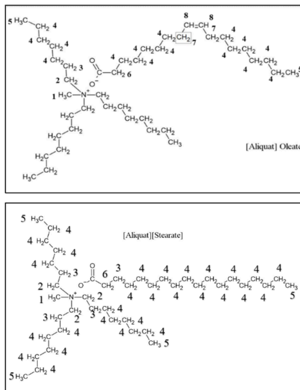
Fig. 1: Structure of [Aliquat][Oleate] and [Aliquat][Stearate]
