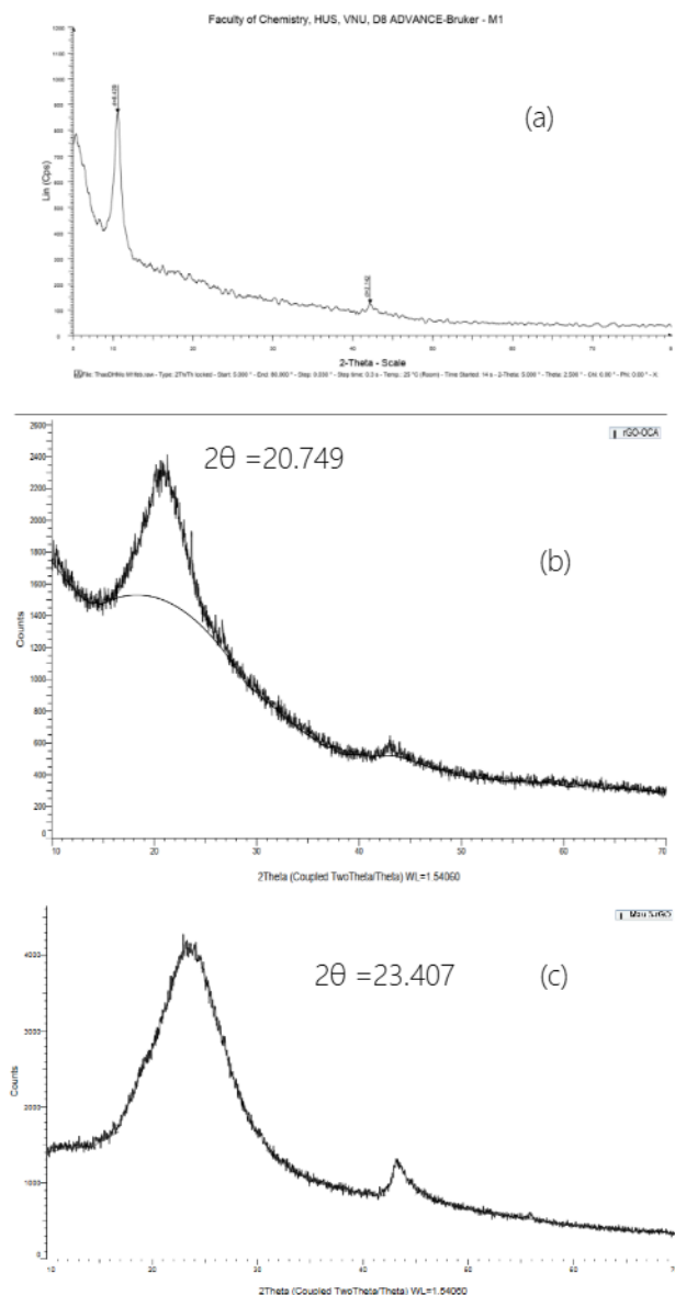
Fig. 2: X-ray patterns of (a) GO, (b) rGO-DoA and (c) rGO
