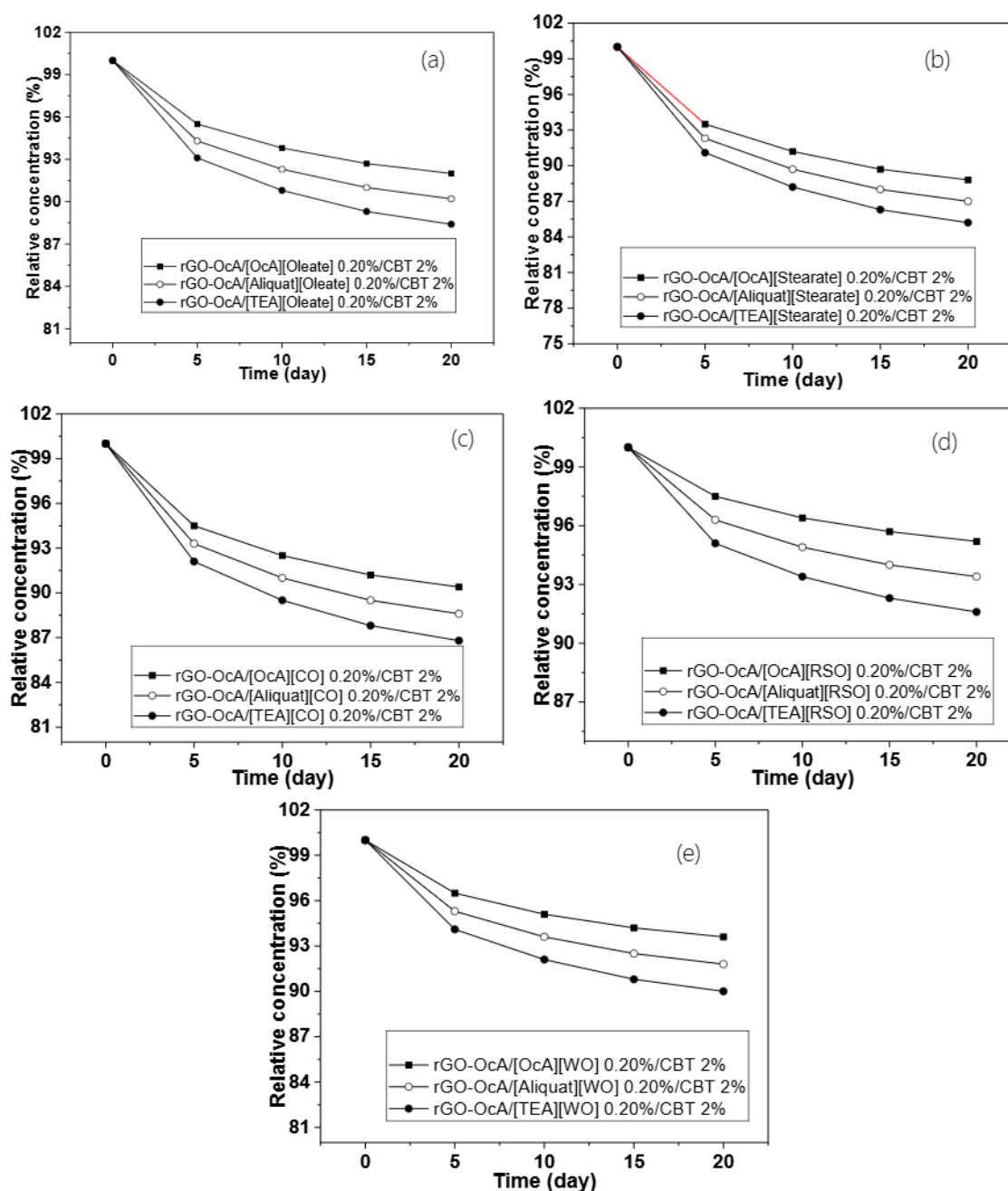
Fig. 4: Influence of ionic liquid cation structure on the dispersion stability of rGO-OcA in lubricants and IL based on anion: (a) oleate; (b) stearate; (c) coconut oil fatty acids; (d) rubber seed oil fatty acids; (e) waste oil fatty acids. (rGO-OcA concentration in IL: 0.004 wt%; IL concentration in lubricant: 2 wt%).
