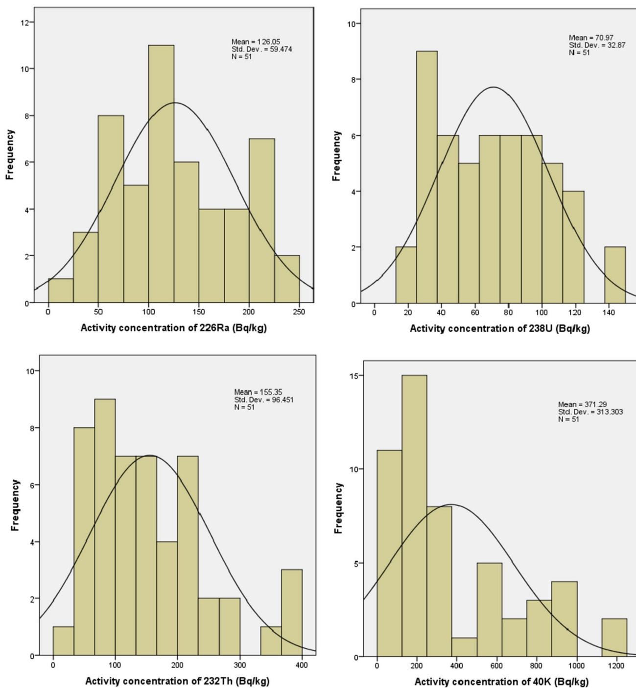
Fig. 2 Distribution curve of ^{226}\text{Ra} , ^{238}\text{U} , ^{232}\text{Th} ( ^{228}\text{Ra} ), and ^{40}\text{K} concentration in the study area
