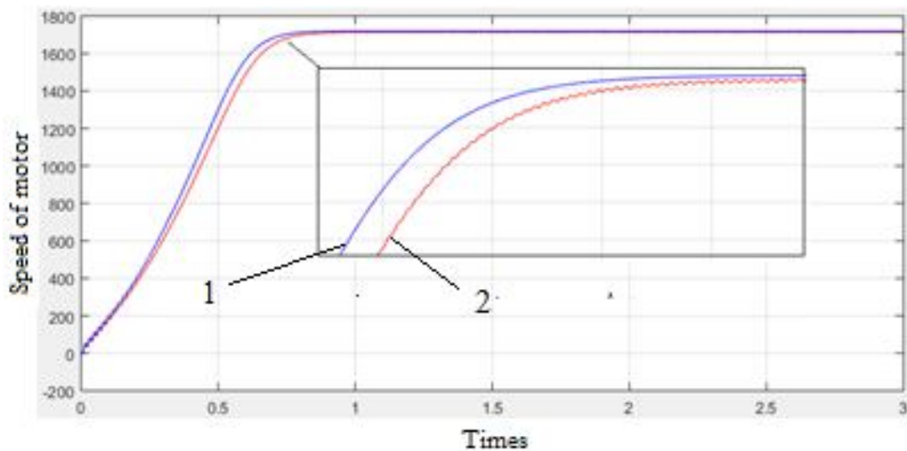
Figure 4. Matlab simulation diagram.
