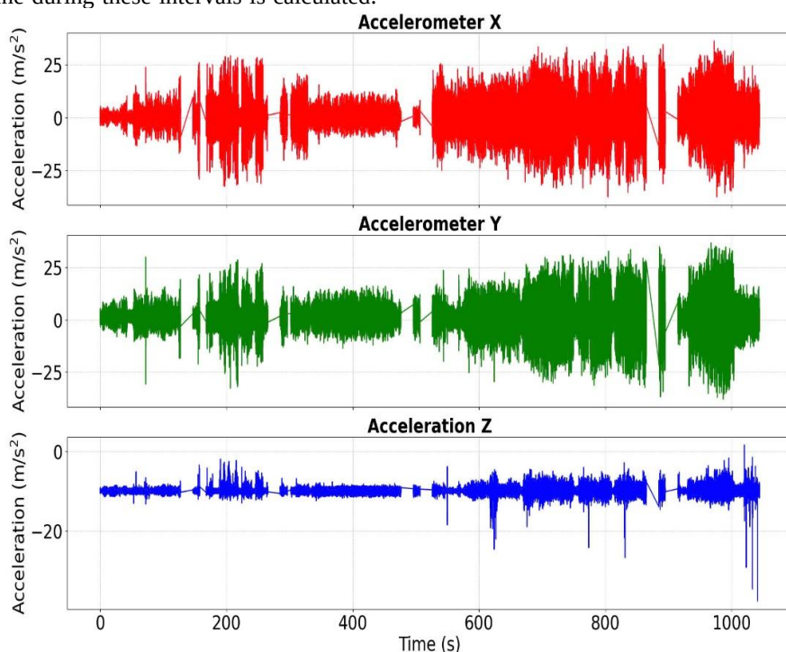
Figure 1. Signal from the accelerometer
