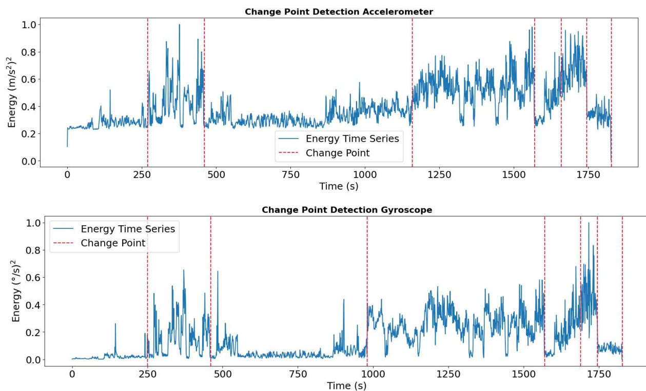
Figure 3. Results of signal segmentation according to drilling state
