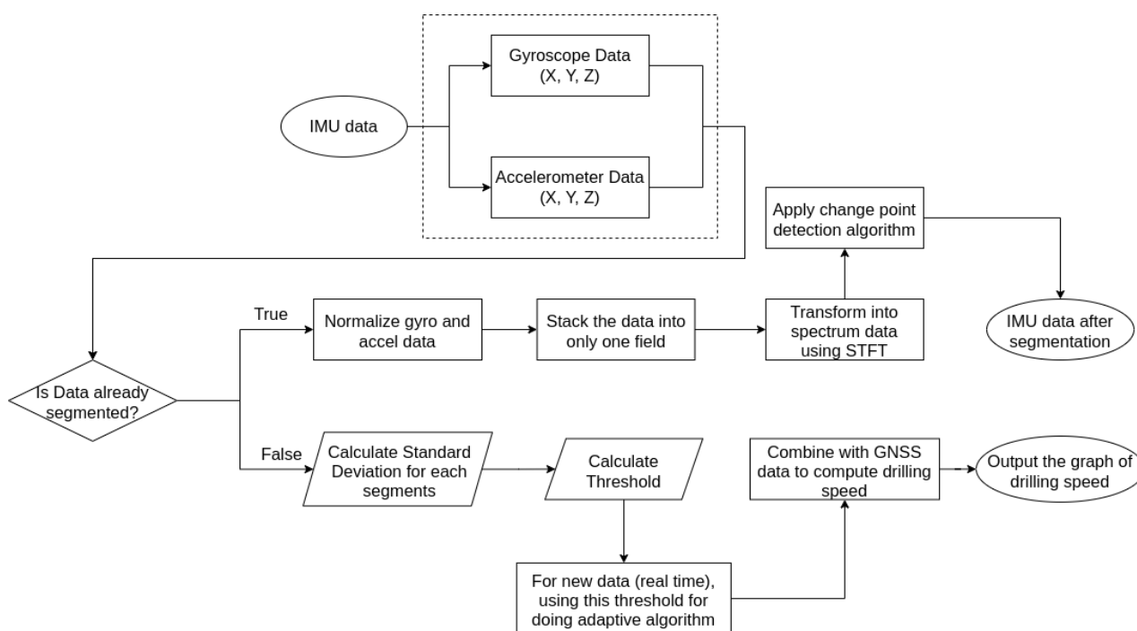
Figure 4. Workflow of computing drilling speed
